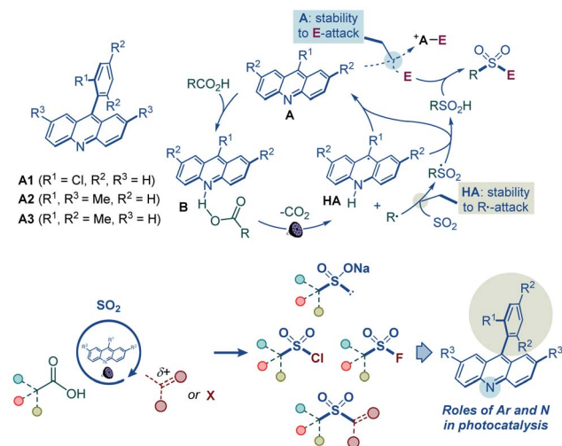
Fig. 2 (A) Decarboxylative construction of sulfones, sulfinates, sulfonyl fluorides and chlorides. (B) Functional group-divergent decarboxylation by acridine photocatalysis.
