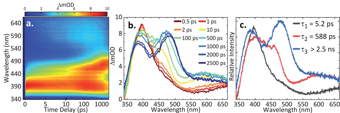
Fig. 3 (a) TA spectra of 1.1 mM AQS in 0.1 M acetate buffer pH 4.9, 0.2 M KCl represented as a false colour map showing changes in optical density ( \Delta\text{MOD} ) with photoexcitation at 330 nm; (b) different time delays ( \Delta t ) chosen for the TA spectra; (c) the corresponding evolution-associated difference spectra (EADS) from the global fit.
