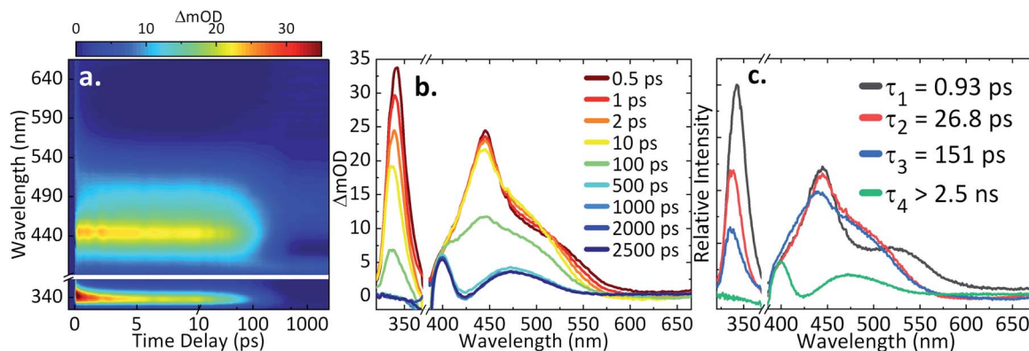
Fig. 5 (a) TA spectra of the electrochemically reduced species ( \text{AH}_2\text{QS} ; 1 mM AQS starting material, 0.1 M acetate buffer pH 4.9, 0.2 M KCl, -0.65 V vs. SCE), represented as a false colour map showing changes in optical density ( \Delta\text{mOD} ) with photoexcitation at 382 nm; (b) different time delays ( \Delta t ) chosen for the TA spectra; (c) the corresponding evolution-associated difference spectra (EADS) from the global fit. Note: the \text{AH}_2\text{QS} data was plotted by masking the spectral region of the pump leakage (370–390 nm).
