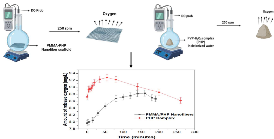
Fig. 5 DO release concentration in deionized water for PHP complex and PMMA/PHP nanofibrous scaffold.
