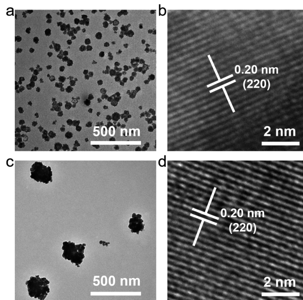
Fig. 1 Morphology of UCBD. TEM images of the \text{Na}_{0.20}\text{Bi}_{0.80}\text{O}_{0.35}\text{F}_{1.91} :10%Yb,2%Er prepared in (a) ethylene glycol and in (c) dimethyl sulfoxide. High resolution TEM images of the \text{Na}_{0.20}\text{Bi}_{0.80}\text{O}_{0.35}\text{F}_{1.91} :10%Yb,2%Er prepared in (b) ethylene glycol and in (d) dimethyl sulfoxide.
