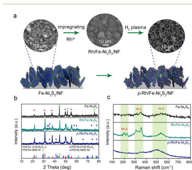
Fig. 1 (a) Schematic illustration of the three-step synthesis of p -Rh/Fe-Ni 3 S 2 /NF with SEM images of Fe-Ni 3 S 2 /NF (left), Rh/Fe-Ni 3 S 2 /NF (middle), and p -Rh/Fe-Ni 3 S 2 /NF (right); (b) XRD patterns and (c) Raman spectra of Fe-Ni 3 S 2 /NF, Rh/Fe-Ni 3 S 2 /NF, and p -Rh/Fe-Ni 3 S 2 /NF.
