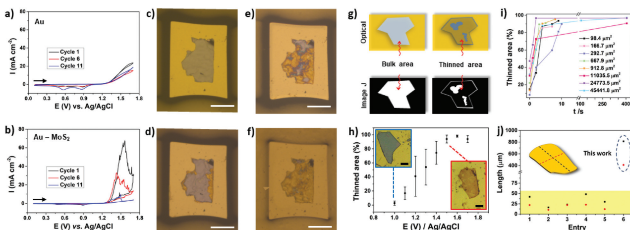
Fig. 3 Cyclic voltammograms (CVs) obtained for (a) Au and (b) Au–MoS 2 ( t flake = 345 nm) electrodes in 0.5 M H 2 SO 4 at 50 mV s -1 . The current was normalized by the geometric area of the electrodes. Stereomicroscope images of the electrodes (Au–MoS 2 ) before the experiment (c) and after cycle 1 (d), cycle 6 (e) and cycle 11 (f). The area and thickness of the MoS 2 flake are 19 714 μm 2 and 345 nm, respectively. The scale bars in c–f are 100 μm. (g) Scheme illustrating the treatment by image J software. (h) Influence of the applied potential on thinned area. Scale bars are 25 μm. (i) Thinned area versus time. (j) Comparison of lateral flake sizes with different works in literature. Red and black dashed lines represent width and length, respectively. Entry: [1], 31 [2, 3], 30 [4] 32 and [5]. 44
