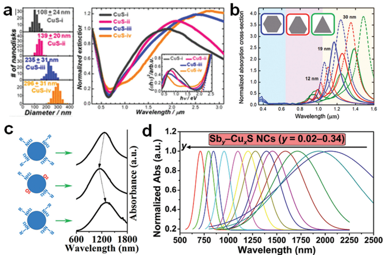
Fig. 11 (a) Optical extinction spectra displaying a red-shift in the longitudinal LSPR peak with increment in the aspect ratio (fixed thickness of ~11 nm). Reproduced from ref. 171 with permission from ACS, copyright 2021; (b) normalized absorption spectra for CuS nanocrystals of hexagonal, triangular, and hexa-triangular shapes for different lateral dimensions: (dashed line) 12 nm, (solid line) 19 nm, and (dash-dotted line) 30 nm displaying red and blue shift in longitudinal and transverse LSPR peak, respectively. Reproduced from ref. 172 with permission from ACS, copyright 2019; (c) tuning of the LSPR peak by the hole density in CuS air exposure and OLA passivation changing. Reproduced from ref. 173 with permission from ACS, copyright 2013; (d) LSPR tuning of \text{Cu}_x\text{S} via \text{Sb}^{3+} doping. Reproduced from ref. 174 with permission from ACS, copyright 2021.
