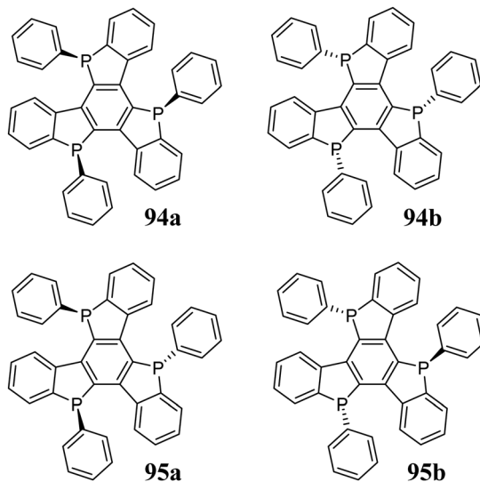
Scheme 33 5,10,15-Triphosphatruxene stereoisomers.
