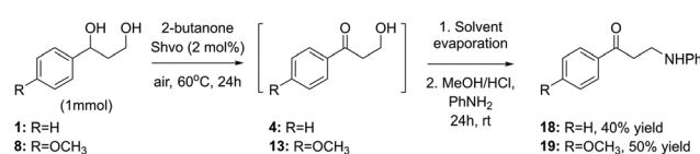
Scheme 7 Two-step diol amination procedure involving solvent replacement.
