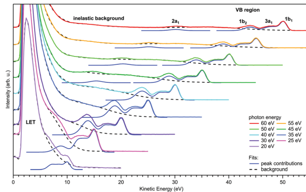
Fig. 3 Valence photoemission spectra from a negatively-biased liquid water microjet at photon energies between 20 and 60 eV; the nominally applied voltage of -50 V has been subtracted from the measured eKE s to produce the eKE scale shown here. Photoelectron peaks due to ionization of the water 1b_1 , 3a_1 , 1b_2 , and 2a_1 orbitals are labeled. Individual contributions are shown by the respective Gaussians. LET denotes the low-energy spectral tail, with intensity maxima clipped here. The dashed black curves represent the contribution from the background signal and the dark blue curves are fits of Gaussians to the peak features. For more details of the fitting procedure, including the description of the background signal we refer to Malerz et al. 34 It is apparent that the peaks are suppressed when the eKE decreases below the critical threshold of \sim 10 eV, while at the same time the inelastic background below the peak increases drastically. Figure is reproduced from Fig. 1 of ref. 34 with permission from the PCCP Owner Societies.
