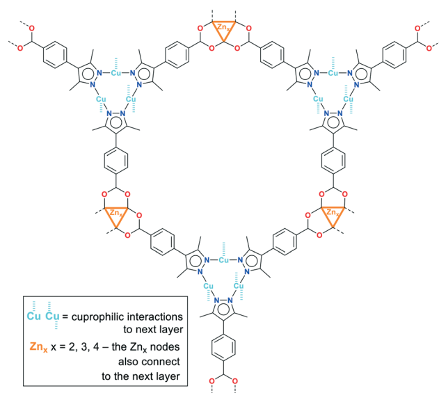
Scheme 2 Common features of the structures of 1–3 with \text{Zn}_x nodes of different nuclearities ( x = 2–4 ) and the trigonal \{\text{Cu}_3(\text{mpbba})_3\}^{3-} nodes giving a hexagonal-ring layer. Both the \text{Zn}_x nodes and the cuprophilic interactions from \{\text{Cu}_3(\text{mpbba})_3\}^{3-} connect to the next layer.
