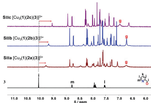
Fig. 3 Comparison of partial ^1\text{H} NMR spectra ( \text{CD}_2\text{Cl}_2 , 600 MHz, 298 K) of ligand 3 , Sla = [\text{Cu}_3(\mathbf{1})(\mathbf{2a})(\mathbf{3})]^{3+} , Slb = [\text{Cu}_3(\mathbf{1})(\mathbf{2b})(\mathbf{3})]^{3+} , Slc = [\text{Cu}_3(\mathbf{1})(\mathbf{2c})(\mathbf{3})]^{3+} .
