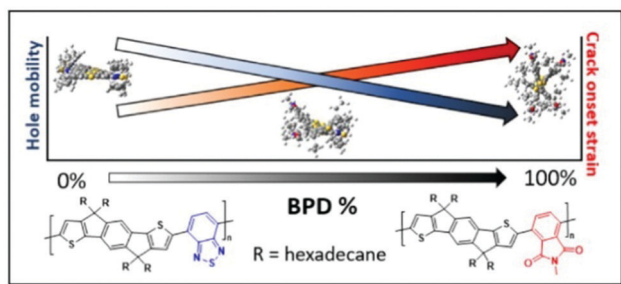
Fig. 10 Chemical structures of PIDTBTB and PIDTBPB in the copolymers with various percentages of BPD unit (along with the respective DFT geometries), and the trends of hole mobility and CoS dependence on the BPD share. Reproduced with permission from American Chemical Society. 38
