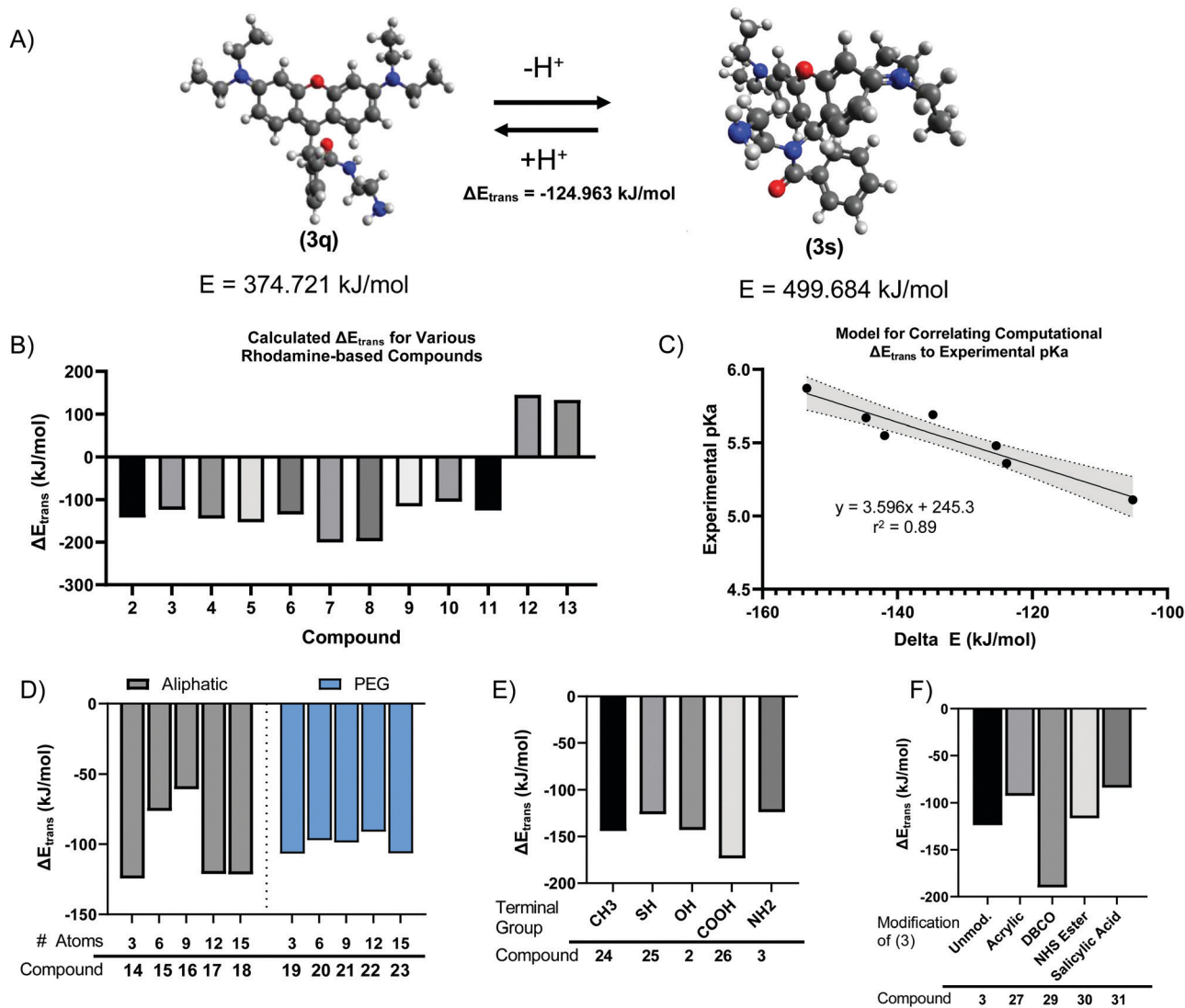
Fig. 3 Ball and stick models of minimum energy geometry-optimized structures of rhodamine 6G (1) modified by 1,2-ethanolamine (3) in its quinone state when protonated (3s) (A). Calculated free energies predict pH-mediated fluorescent properties because of a favorable transition to the quinone state when protonated (B) which correlate with experimental pK a values (C, shaded area represents 95% confidence interval of the regression). Computational interrogation of theoretical compounds 14–23 to investigate aliphatic chain length-dependence of the energy difference between the spirolactam and quinone forms (D, 14–18) and effect of ethylene glycol substitution of the same length (D, 19–23). Amide derivatives of (1) with various terminal functional groups are energetically favorable (E). Amide derivatives, such as (3), can be further modified favorably to impart specific chemical functionality (F) while maintaining energetically favorable pH-dependent fluorescence.
