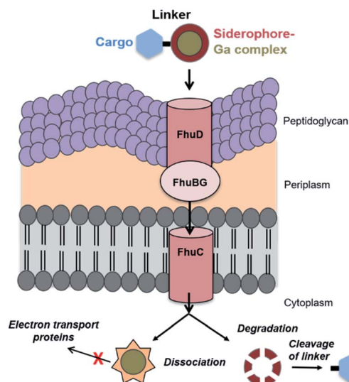
Fig. 1 Proposed transport internalization pathway for ferrichrome based Galbofloxacin in wt S. aureus using active transmembrane transport.
