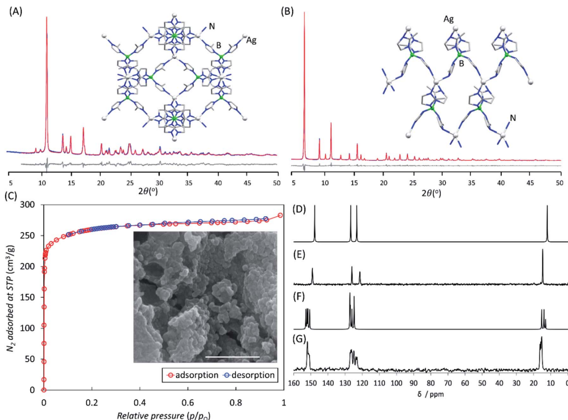
Fig. 6 (A) Rietveld refinement of Ag-BIF-3 with difference plot shown in grey. (B) Rietveld refinement of Ag-BIF-2 with difference plot shown in grey. (C) BET adsorption plot for Ag-BIF-3 showing a surface area of 1020 \text{ m}^2 \text{ g}^{-1} and a SEM image of a representative sample (scale-bar 1 \mu\text{m} ). Comparison of measured and simulated ^{13}\text{C} CP-MA ssNMR spectra for silver-based BIFs: (D) calculated for Ag-BIF-3, (E) measured for Ag-BIF-3, (F) calculated for Ag-BIF-2 and (G) measured for Ag-BIF-2.
