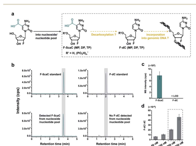
Fig. 5 F-5caC was not decarboxylated to F-dC in soluble nucleoside/nucleotide pool. (a) Schematic overview of the assumed pathway of decarboxylation of F-5caC in nucleoside/nucleotide soluble pool. F-5caC (MP, DP, and TP) and F-dC (MP, DP, and TP) refer to the form of nucleoside, monophosphate, diphosphate, and triphosphate, respectively. (b) Extracted-ion chromatograms for monitoring F-5caC and F-dC in the soluble pool. (c) Quantitative data of F-5caC and F-dC in the soluble pool after feeding 300 \mu M of F-5caC for 3 d. (d) Quantification of F-dC level in genomic DNA after feeding of F-dC with diverse concentrations to HEK293T cells for 3 d.
