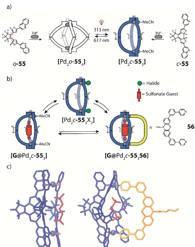
Fig. 27 (a) Photoswitching a quinolin-substituted ligand with dithienylethene (DTE) backbone allows cycling between a [Pd 2 L 4 ] cage and [Pd 2 L 3 Solv 2 ] bowl-shaped structure; (b) guest binding can be modulated by changing the host's charge from 4+ to 2+ by adding halide anions as trigger or by changing the cavity size via a fourth ligand (yellow); (c) X-ray crystal structures of host-guest complexes of the bowl and unprecedented [Pd 2 L 3 ] heteroleptic cage.
