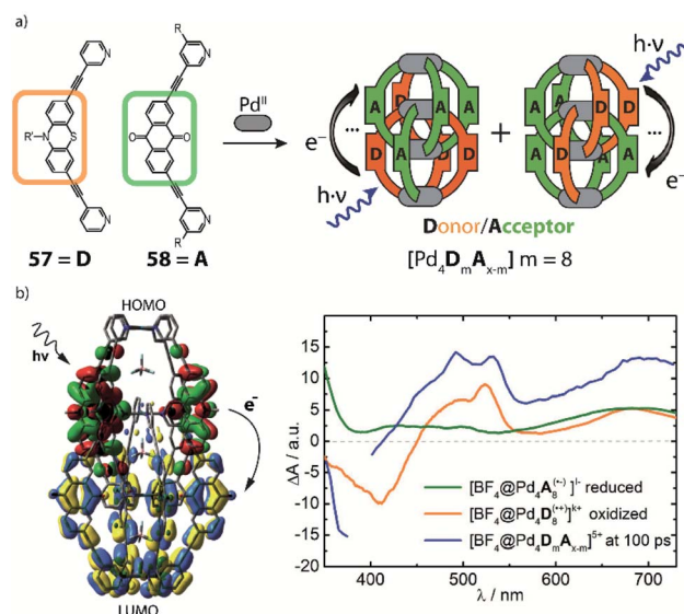
Fig. 28 (a) Phenothiazine-based donors (D) and anthraquinone-based acceptors (A) were implemented in ligands whose combination with Pd II cations leads to a statistical mixture of mixed-ligand interpenetrated double-cages which show (b) light-triggered charge separation as monitored by transient absorption and spectroelectrochemistry.
