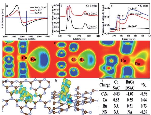
Fig. 3 Evidence of charge transfer. (a) EPR spectra, (b and c) NEXAFS results: (b) Co L-edge and (c) N K-edge. (d–f) Electronic function location (EFL) for Ru and Co atoms on (d) graphitic N, (e) pyridinic N and (f) pyrrolic N species. (g and h) Charge density differences over (g) RuCo DSAC and (h) RuCo DSAC@N 2 . (i) Charge variation during N 2 adsorption on RuCo DSAC and Co SAC samples.
