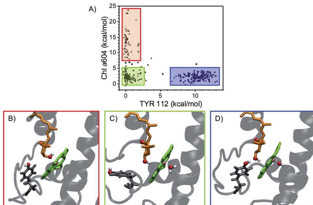
Fig. 6 The N1 binding pocket assumes different conformations. (A) Electrostatic interaction energy of N1 neoanthin of LHCII with either TYR112 (x-axis) or Chl a604 (y-axis). Three different clusters of data points (each point represents a single MD snapshot) can be visualized in the scatter plot, representing either no strong interaction (enclosed in the green rectangle), preferential interaction with Chl a604 (red) or preferential HB to TYR112 (blue). The latter cluster is also the most abundant. (B–D) Conformations of the N1 binding pocket characterized by distinct interaction patterns and corresponding to three MD snapshots representative of the clusters shown in (A), with the same color code adopted for the surrounding rectangles. Neoanthin is shown in orange, Chl a604 in green, TYR112 in gray, and the protein in transparent gray. The water molecule coordinating Chl a604 is also shown, if present. The polar oxygen and hydrogen atoms are highlighted in red and white, respectively, whereas the Mg of Chl a604 is highlighted in pink. In (B), the –OH group of neoanthin interacts strongly with the Mg of Chl a604, which lacks the coordinating water molecule. In (C), neoanthin shows weak interactions with both Chl a604 (which is coordinated by a water molecule) and TYR112. In (D), neoanthin forms a strong HB with TYR112.
