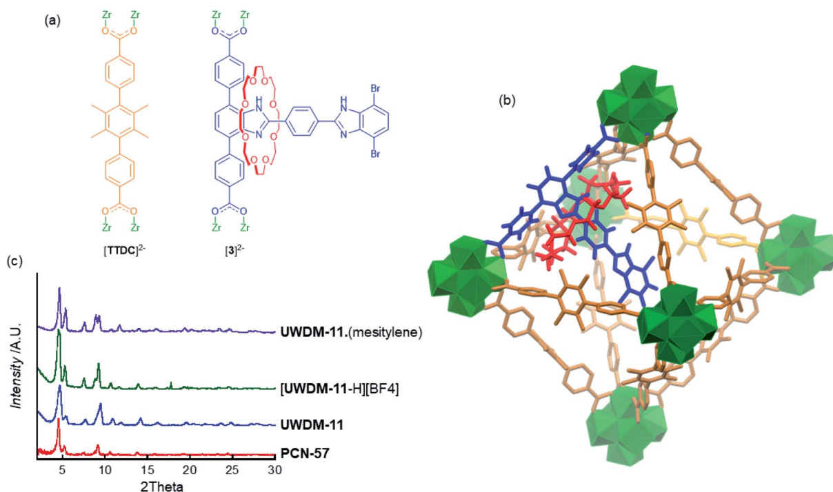
Fig. 3 (a) The two linkers used to construct the multivariate MOF UWDM-11 ; primary linker [TTDC] 2- and [2]rotaxane [3] 2- . (b) A Molecular Studio (Forcite) geometry-optimised model of the octahedral cavity in UWDM-11 ; MIM axle = blue, 24C8 macrocycle = red, primary [TTDC] 2- linkers = orange and [Zr 6 O 4 (OH) 4 ] 12+ nodes = green. (c) PXRD of PCN-57 and various versions of UWDM-11 .
