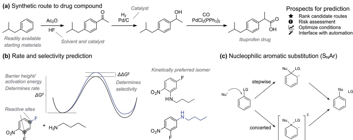
Fig. 1 (a) Example of synthetic route to a drug compound. Prospects for AI-assisted route design. (b) Accurate prediction of reaction barriers gives both rate and selectivity. (c) The nucleophilic aromatic substitution ( S_NAr ) reaction.
