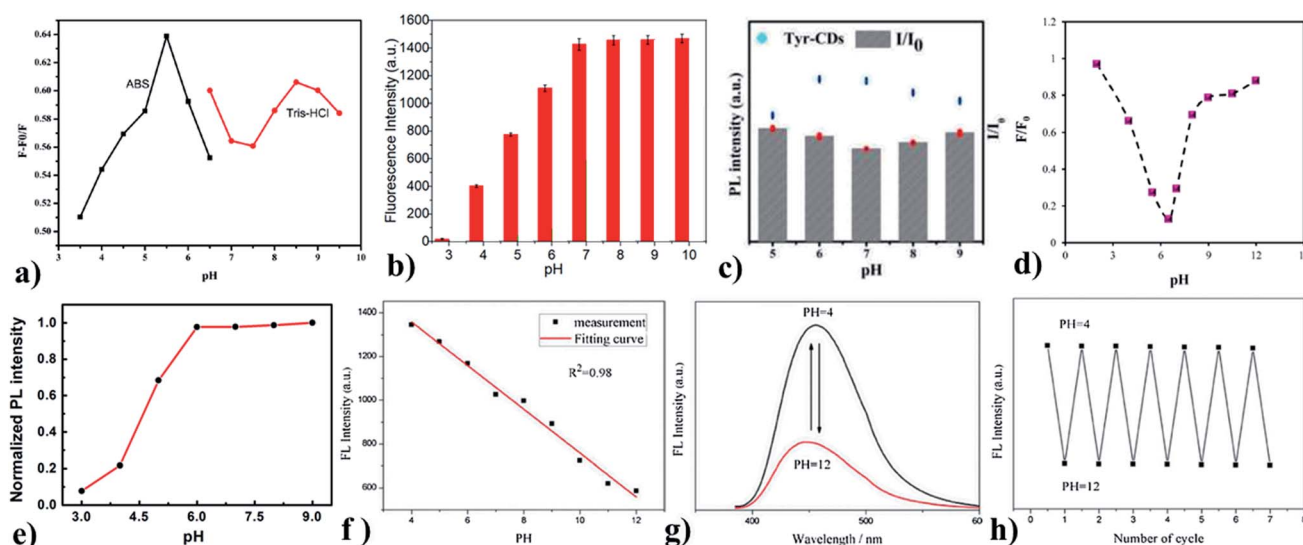
Fig. 4 (a) and (b) pH vs. change in fluorescence intensity of Gly-GQDs, (c) pH vs. change in the fluorescence intensity of Tyr-CDs, (d) pH vs. change in fluorescence intensity of Val-GQDs, (e) pH vs. change in the fluorescence intensity of L-CQDs, (f) pH vs. change in the fluorescence intensity for BR buffer, (g) pH vs. fluorescence spectra of Trp-GQDs, (h) Response of reversible fluorescence for varying pH cycles. In the figure, (a) has been reproduced from ref. 79 with permission from Elsevier, copyright 2017; (b) has been reproduced from ref. 33 with permission from Elsevier, copyright 2021; (c) has been reproduced from ref. 80 with permission from Elsevier, copyright 2015; (d) has been reproduced from ref. 34 with permission from Elsevier, copyright 2017; (e) has been reproduced from ref. 81 with permission from Springer, copyright 2016; (f)–(h) have been reproduced from ref. 84 with permission from Elsevier, copyright 2019.
