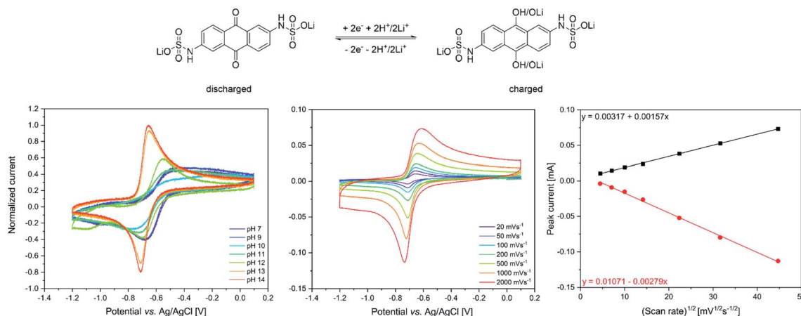
Fig. 2 Top: schematic representation of the redox chemistry of the LiAQS. Bottom: cyclic voltammetry of a 50 mM LiAQS in 0.1 M lithium chloride solution. Scan direction: 0 V to -1.2 \text{ V} and back to 0 V. For each condition five scans were carried out and the third is shown. (left) pH-dependent investigation utilizing lithium hydroxide for adjusting the pH-value with a scan speed of 100 \text{ mVs}^{-1} , (middle) CV at different scan speeds at a pH-value of 14, (right) plot of the peak current for the oxidation (black) and reduction process (red) vs. the square root of the scan speed at a pH-value of 14.
