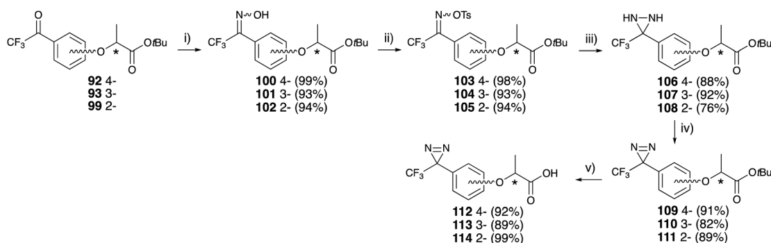
Fig. 15 Asymmetric synthesis of trifluoromethyldiazirinyl lactisole derivatives. (i) \text{H}_2\text{NOH}\cdot\text{HCl} , pyridine, EtOH, 60 °C, 12 h, (ii) \text{CH}_3\text{CH}(\text{O}^*\text{Me})\text{CO}_2\text{Me} ( 79 ), \text{PPh}_3 , \text{CH}_2\text{Cl}_2 , 0 °C, 10 min, (iii) \text{DEAD} , rt, 8 h, (iv) \text{K}_2\text{CO}_3 , MeOH, \text{H}_2\text{O} , reflux, 2 h, (v) t\text{-BuBr} , \text{K}_2\text{CO}_3 , TBAB, DMA, 55 °C, 5 h, (vi) \text{CH}_3\text{I} , \text{NaHCO}_3 , \text{CH}_3\text{CN} , \text{H}_2\text{O} , rt, 24 h, (vii) (1) \text{TMS-CF}_3 , \text{K}_2\text{CO}_3 , DMF, rt, 4 h, (2) 1 M \text{HCl} , rt, 4 h, (3) Dess–Martin periodinane, \text{CH}_2\text{Cl}_2 , rt, 3 h.
