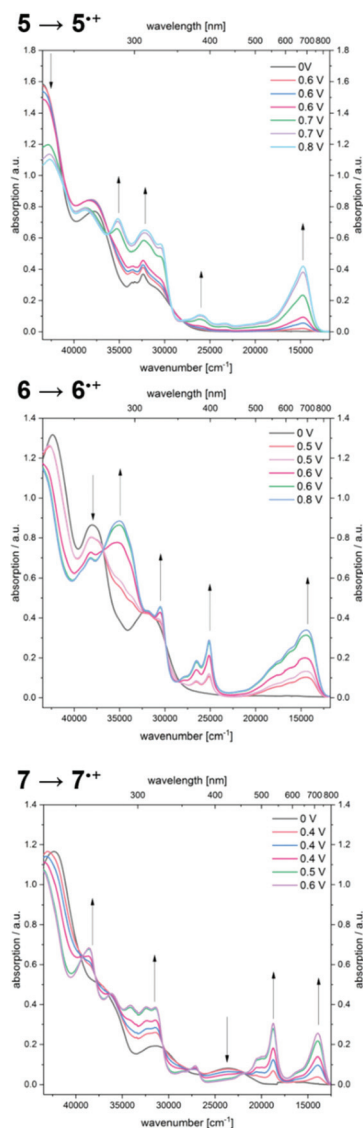
Fig. 7 UV/Vis spectroelectrochemical measurements of compounds 5 , 6 , and 7 forming the corresponding radical cations 5^+ , 6^+ , and 7^+ ( \text{CH}_2\text{Cl}_2 , T = 293 K; electrolyte 0.1 M [ ^t\text{Bu}_4\text{N} ][PF 6 ]; Pt working electrode, Pt counter electrode and Ag/AgCl pseudo reference electrode).
