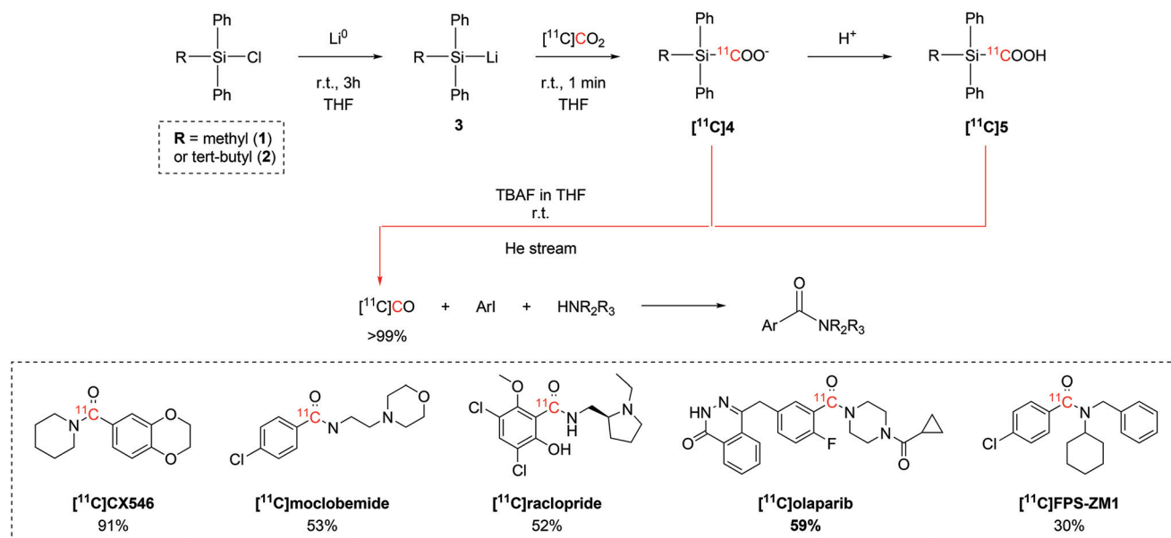
Scheme 2 ^{11}\text{C} CO 2 -to- ^{11}\text{C} CO conversion via ^{11}\text{C} -silanecarboxylate derivatives, ^{11}\text{C} -carbonylation of aryl iodides and biologically-active molecules successfully synthesized with the produced ^{11}\text{C} CO. 37–39
