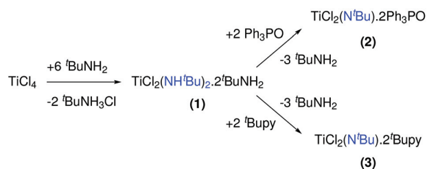
Fig. 4 Reactions of titanium chloride with tert butylamine and thiphenylphosphine oxide or tert butylpyridine.
