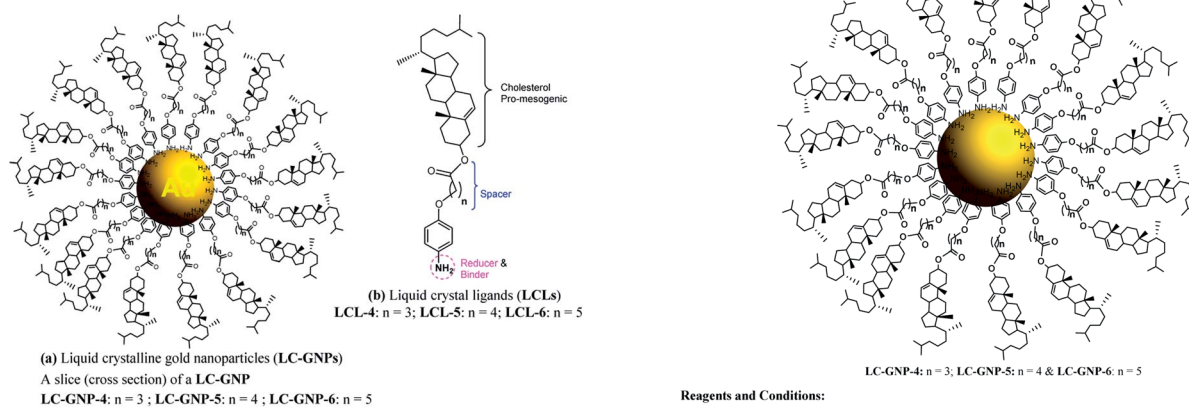
Fig. 1 Schematic illustration of the newly synthesized LC-GNP conjugates (a), where LC ligands (b), featuring reducing and binding sites, a spacer of varying length and parity and a pro-mesogenic core, are spherically grafted onto the surface of a central gold atom.
