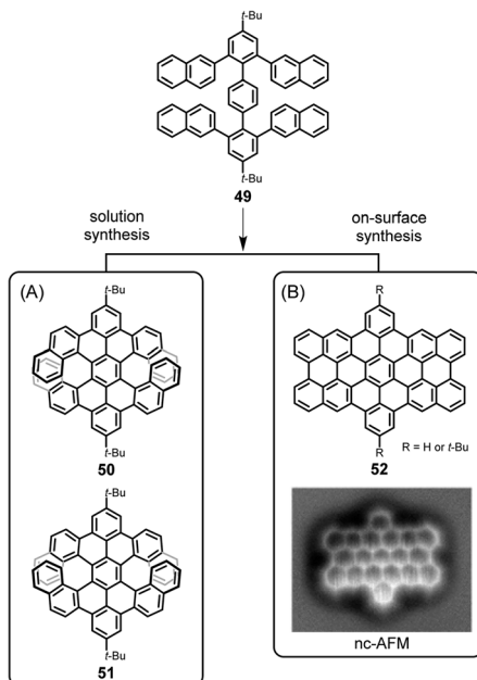
Fig. 7 Different cyclodehydrogenation pathways for solution and on-surface syntheses: (A) double [7]helicenes 50 and 51 , and (B) benzo-fused periacyene 52 . Inset in (B): constant-height noncontact AFM (nc-AFM) image of 52 on Cu(110). 124 Copyright 2019. Adapted with permission from the American Chemical Society.
