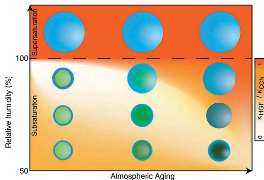
Fig. 34 Schematics of the water uptake processes of SOA particles in the atmosphere. Subsaturation swelling ( k_{\text{HGF}} ) can vary dramatically with minor differences in supersaturated droplet activation ( k_{\text{CCN}} ); consequently, particles can have very different direct and indirect climate effects. The background color scale indicates the ratio of these parameters under the given subsaturated and supersaturated conditions, whereas the darkness of the green color in particles denotes their atmospheric age. The contrast is the largest when adsorption is the dominant water uptake mechanism even at high RH. This is the case for low O : C SOA particles on the left. With increasing oxidation, i.e. , increasing atmospheric age of the particles, the solubility increases and the dissolution RH decreases, decreasing the discrepancy between the k_{\text{HGF}} and k_{\text{CCN}} values. Reproduced from ref. 326 under Create Commons License (CC BY-NC-ND 4.0) from the American Geophysical Union, © The Authors, 2015.
