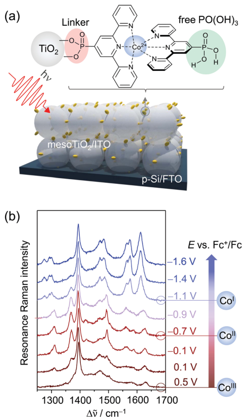
Fig. 7 (a) Phosponic acid modified Co bisterpyridine adsorbed on mesoporous \text{TiO}_2 or ITO (meso \text{TiO}_2 /mesoITO). (b) EC-RR spectra revealing the reduction of adsorbed CotpyP on mesoITO from \text{Co}^{\text{III}} to \text{Co}^{\text{II}} to \text{Co}^{\text{I}} in the potential range from 0.5 V_{\text{Fc}^+/\text{Fc}} to -1.6 V_{\text{Fc}^+/\text{Fc}} (514 nm excitation, acetonitrile with 0.1 M TBABF 4 ). Graph redrawn from ref. 71.
