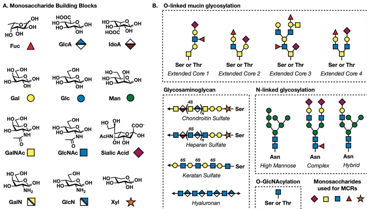
Fig. 1 (A) Common mammalian monosaccharide building blocks and their geometric codes. (B) Core structures for O-linked mucin, N-linked, GAG, and O-GlcNAc glycosylation.
