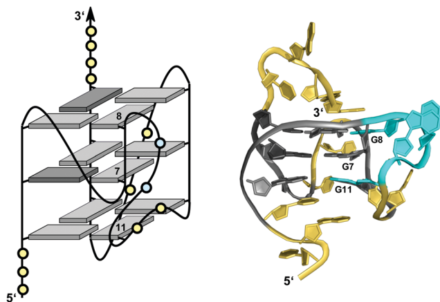
Fig. 14 Schematic representation (left) and three-dimensional solution structure (right) of a G-quadruplex with a D-shaped loop derived from a VEGF aptamer with locked LNA G residues in K + solution (10 mM KP i + 40 mM KCl, pH 7.0; T m = 52 °C; PDB 2M53); 26 anti -guanosines and LNA analogs of the G-core are colored in light and dark grey, respectively; loop and flanking residues, yellow; residues of D-shaped loop, cyan.
