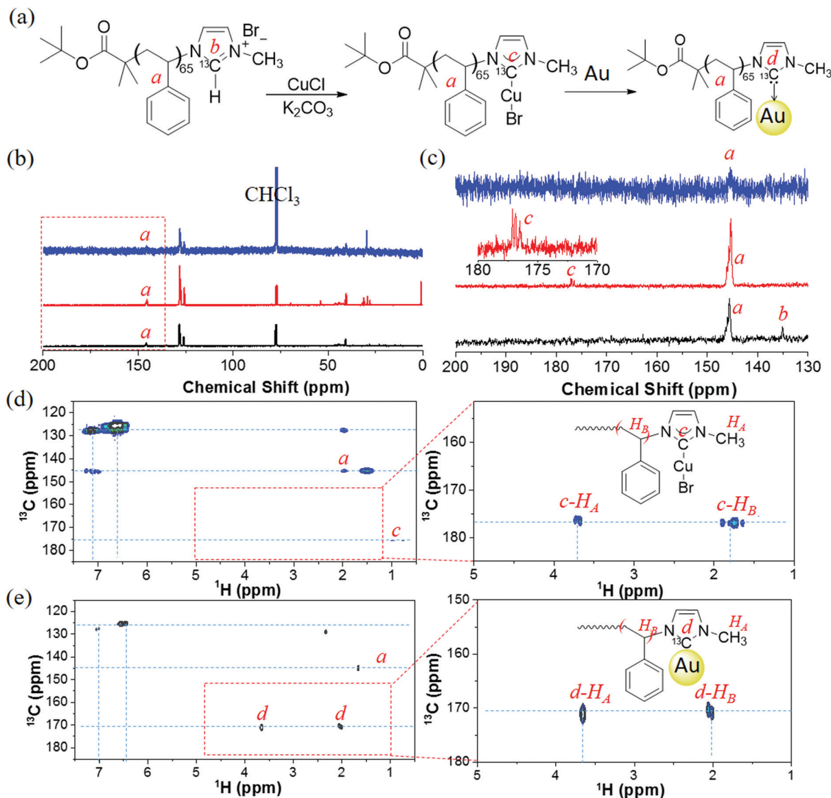
Fig. 3 (a) Synthesis of ^{13}\text{C} -labeled \text{PS}_{65}\text{-}^{13}\text{C}\text{-NHC-Au} using ^{13}\text{C} -Im. (b and c) ^{13}\text{C} NMR spectra of \text{PS}_{65}\text{-}^{13}\text{C}\text{-Im} (black, bottom), \text{PS}_{65}\text{-}^{13}\text{C}\text{-NHC-Cu(I)} (red, middle) and \text{PS}_{65}\text{-}^{13}\text{C}\text{-NHC-Au} (blue, top) in \text{CDCl}_3 . ^{13}\text{C} NMR spectra in (b) in the range of 130–200 ppm is zoomed in (c). (d) 2D HMBC spectrum of non-labeled \text{PS}_{65}\text{-NHC-Cu(I)} . (e) 2D HMBC spectrum of ^{13}\text{C} -labeled \text{PS}_{65}\text{-}^{13}\text{C}\text{-NHC-Au} .
