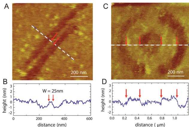
Fig. 24 (A) AFM image of a nanoribbon fabricated on a graphene flake with thickness \sim 1\text{ nm} . The width and length of the ribbon are 25 and 800 nm, respectively. (B) Height profile along the dashed line in (a). (C) A nanoring (inner radius \sim 160\text{ nm} , outer radius \sim 380\text{ nm} ) patterned on a graphene flake. Two long trenches, not shown in the picture, were subsequently drawn from the circumference of the ring outward to the edges of the flake to electrically isolate the ring device. (D) Height profile along the dashed line in (c). Reproduced from ref. 152 with permission from the AIP Publishing.
