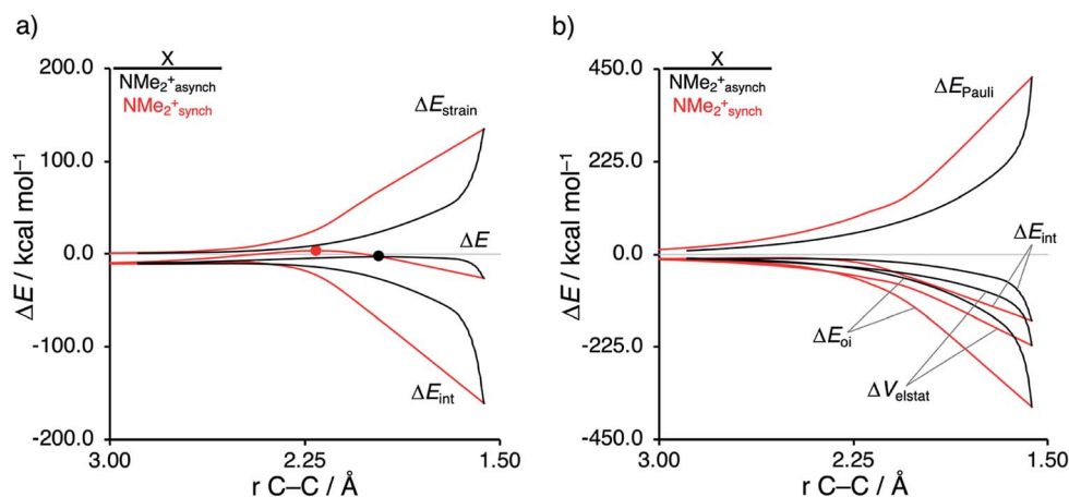
Fig. 5 (a) Activation strain analyses and (b) energy decomposition analyses of the asynchronous (black) and constrained synchronous (red) Diels–Alder reactions between CP and \text{NMe}_2^+ going from the reactants to the product, where the transition states are indicated with a dot and the energy values are projected onto the shorter newly forming \text{C}_{\text{CP}}\cdots\text{C}_{\beta} bond between CP and \text{NMe}_2^+ , computed at ZORA-M06-2X/TZ2P//M06-2X/def2-TZVP for \text{NMe}_2^+_{\text{asynch}} and ZORA-M06-2X/TZ2P for \text{NMe}_2^+_{\text{synch}} .
