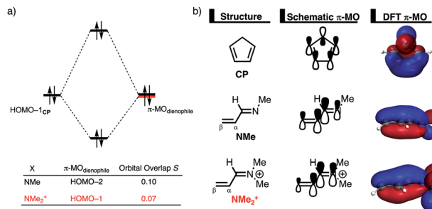
Fig. 4 Molecular orbital diagrams of the key orbital interactions of the Diels–Alder reactions between CP and NMe and \text{NMe}_2^+ : (a) most significant occupied orbital overlaps and (b) 3D plots of the involved occupied orbitals (isovalue = 0.03 \text{ au}^{-3/2} ). All data were computed at consistent geometries with a \text{C}_{\text{CP}}\cdots\text{C}_{\beta} bond length between CP and the dienophile of 2.125 Å at ZORA-M06-2X/TZ2P//M06-2X/def2-TZVP.
