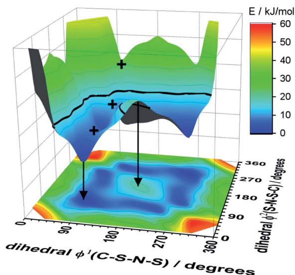
Fig. 4 The upper part of the image is the 3D potential energy surface (PES) of the [N(\text{Tf})_2]^- anion and the lower surface the 2D projection. Plus symbols mark selected transition states. The arrows indicate how a local minimum and maximum are mapped on the 2D projection. The bold line at 15 \text{ kJ mol}^{-1} will facilitate comparison with other surfaces. The lowest energy conformer is taken as zero reference.
