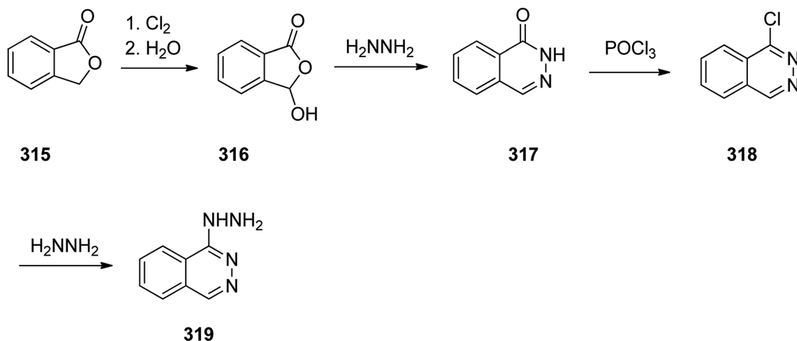
Scheme 43 Synthesis of hydalazine 319.
