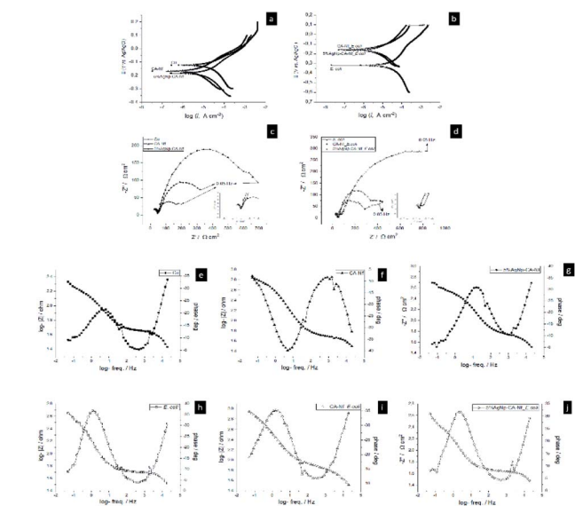
Fig. 9 Abiotic and biotic corrosion set ups potentiodynamic polarization curves (a and b), Nyquist plots (c and d) and Bode plots (e-j).
