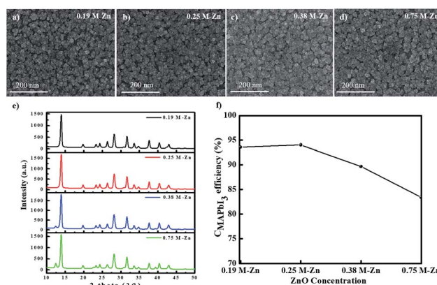
Fig. 6 SEM surface morphologies of the \text{MAPbI}_3 perovskite layers fabricated on \text{ZnO} ((a) 0.19 M-Zn, (b) 0.25 M-Zn, (c) 0.38 M-Zn, (d) 0.75 M-Zn) over the \text{c-TiO}_2 layers under two SDC and three SSIER cycles and (e) the XRD patterns of these \text{MAPbI}_3 perovskite layers and (f) the C_{\text{MAPbI}_3} values for various thicknesses of ZnO layers.
