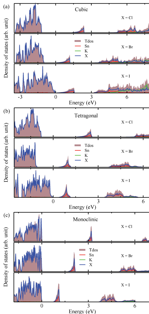
Fig. 2 Total and atomic resolved electronic density of states in \text{K}_2\text{SnX}_6 (X = I, Br, Cl) in (a) cubic, (b) tetragonal and (c) monoclinic phases, calculated using the HSE functional with the SOC effect.
