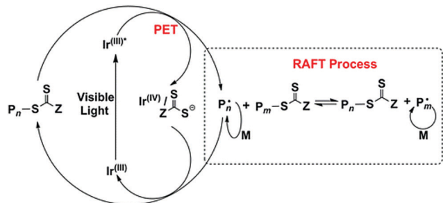
Fig. 2 Mechanism of PET-RAFT using fac -[Ir(ppy) 3 ] as a photoredox catalyst. Adapted from ref. 33 with permission. Copyright (2014) American Chemical Society.
