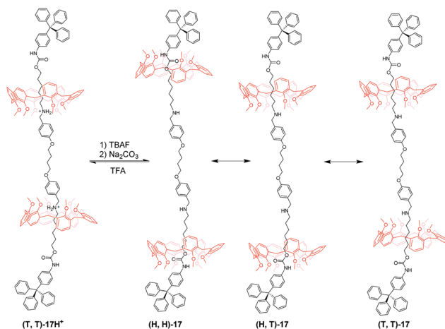
Fig. 17 pH-Controlled calix[6]arene-based [3]rotaxane 17 .
