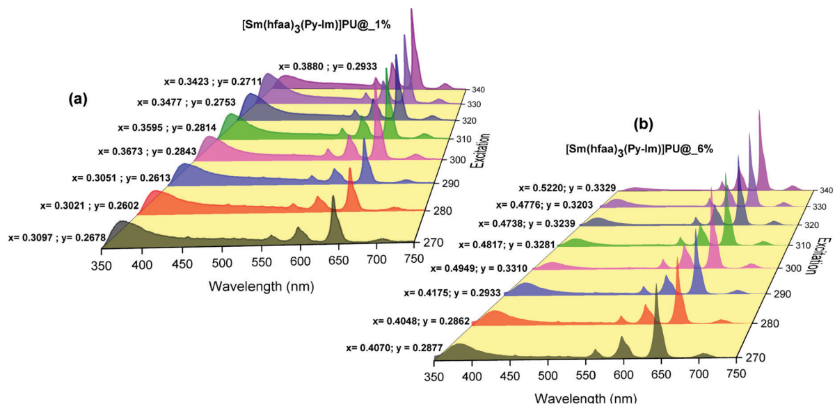
Fig. 10 Corrected emission spectra of hybrid thin films at different excitation wavelengths at RT. The values are CIE (x,y) color coordinates obtained.
