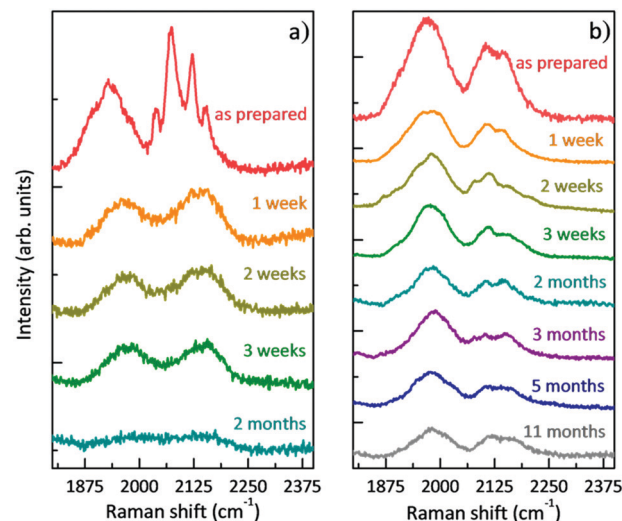
Fig. 4 Evolution in time of the SERS spectra: (a) polyynes solution of PVA1% with Ag colloid (L-1%_Ag) and (b) free-standing nanocomposite of Ag/PVA1%/polyynes (S-1%_Ag).
