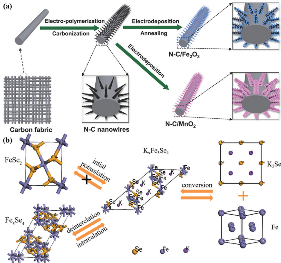
Fig. 10 Schematic of N-doped carbon nanowires@MnO 2 and N-doped carbon nanowires@Fe 2 O 3 . (a). (Reproduced with permission. 147 Copyright 2018, Wiley-VCH.) Schematic for the potassium storage reaction mechanism (b). (Reproduced with permission. 157 Copyright 2019, Wiley-VCH.)
