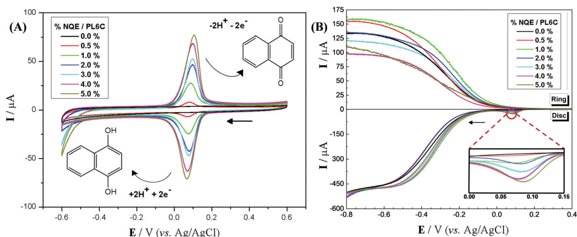
Fig. 1 (A) Cyclic voltammetry on an RRDE with different percentages of NQE and PL6C matrix in \text{N}_2 -saturated 0.1 mol \text{L}^{-1} \text{H}_2\text{SO}_4 (pH 2), at a scan rate of 50 \text{mV s}^{-1} . (B) Comparative linear sweep voltammogram of Printex L6 carbon microlayers and different percentages of NQE on the RRDE electrode in \text{O}_2 -saturated 0.1 mol \text{L}^{-1} \text{H}_2\text{SO}_4 (pH 2), at 900 rpm and a 5 \text{mV s}^{-1} scan rate. The inset between 0.0 and 0.15 \text{V}_{\text{Ag}/\text{AgCl}} is related to reduced quinone, while the arrows indicate the direction of the scan.
