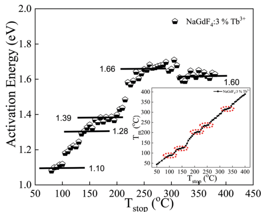
Fig. 12 Activation energy (eV) vs. T_{\text{stop}} ( ^{\circ}\text{C} ) plot resulting from the IR method after the T_m - T_{\text{stop}} procedure for the NaGdF 4 :3% Tb 3+ phosphor irradiated with gamma radiation of 10 kGy doses. A plot of T_m as a function of T_{\text{stop}} for the NaGdF 4 :3% Tb 3+ phosphor as an inset image.
