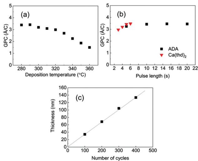
Fig. 2 ALD/MLD parameters for the \text{Ca}(\text{thd})_2 + \text{ADA} process: GPC versus (a) deposition temperature and (b) precursor pulse lengths and (c) film thickness versus number of ALD/MLD cycles; in (a) and (b) 200 ALD/MLD cycles; in (b) and (c) deposition temperature 290 °C; in (a) & (c) pulse/purge sequence: \text{Ca}(\text{thd})_2 5 s, \text{N}_2 5 s, ADA 10 s, and \text{N}_2 30 s.
